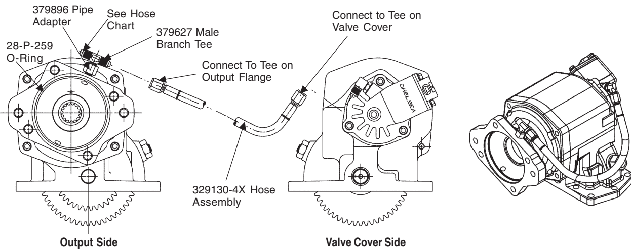
Pressure Hose Chart (Transmission to P.T.O.)
